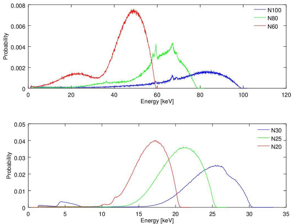
Figure 4: In the image, it can be observed the tube X-Ray spectra qualities N20, N25, N30, N60, N80, and N100.
