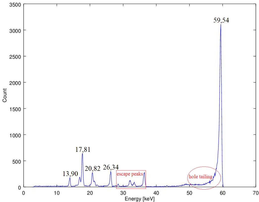
Figure 3: Sealed Am-241 source measured spectrum hole tailing.
