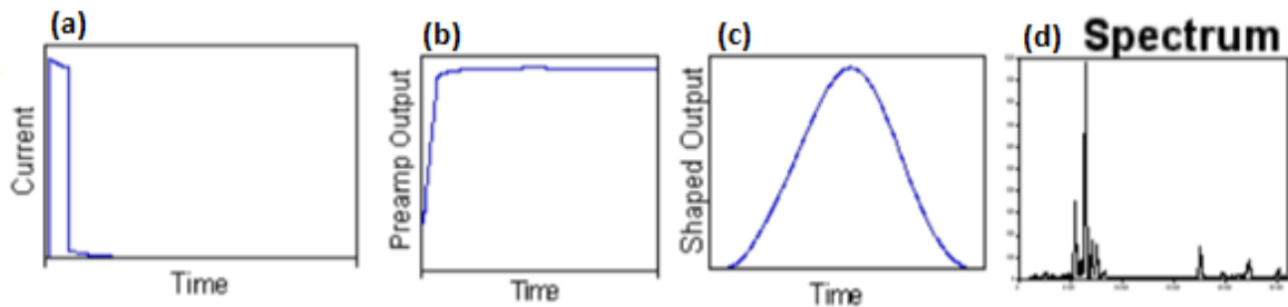
Figure 2: In the image, there is a description of the signal behavior in the spectrometry system. Letter (a) there is the input signal in the preamplifier, (b) the input signal of the amplifier, (c) the input signal of the MCA, and (d) the output signal from MCA that is the spectrum. Image partially reproduced from the manufacturer manual (Amptek 2019).
