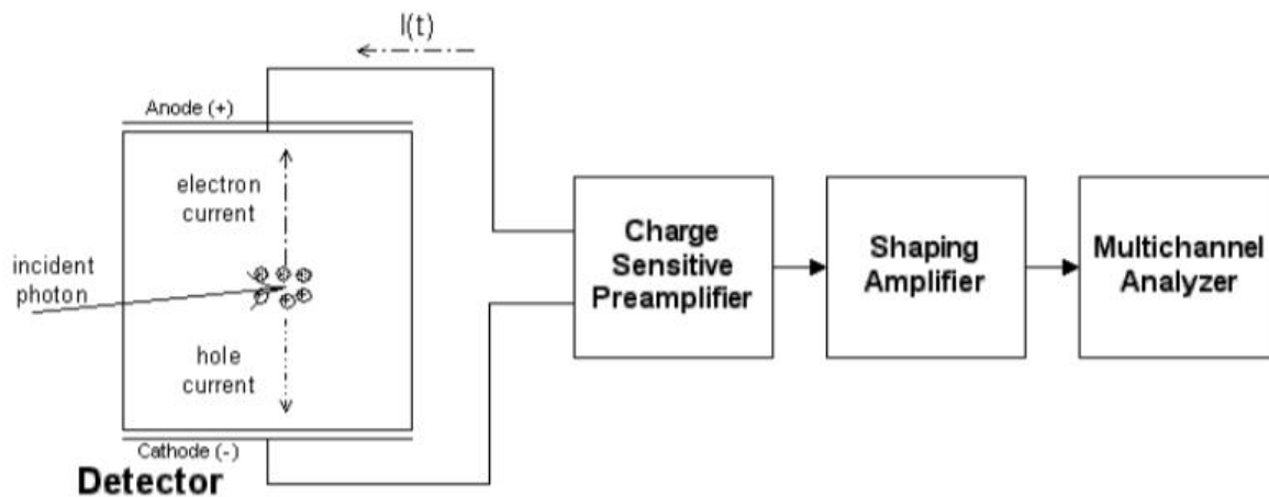
Figure 1: There is in the image a summarized description of a traditional spectrometry system. Image partially reproduced from the manufacturer manual (Amptek 2019).
